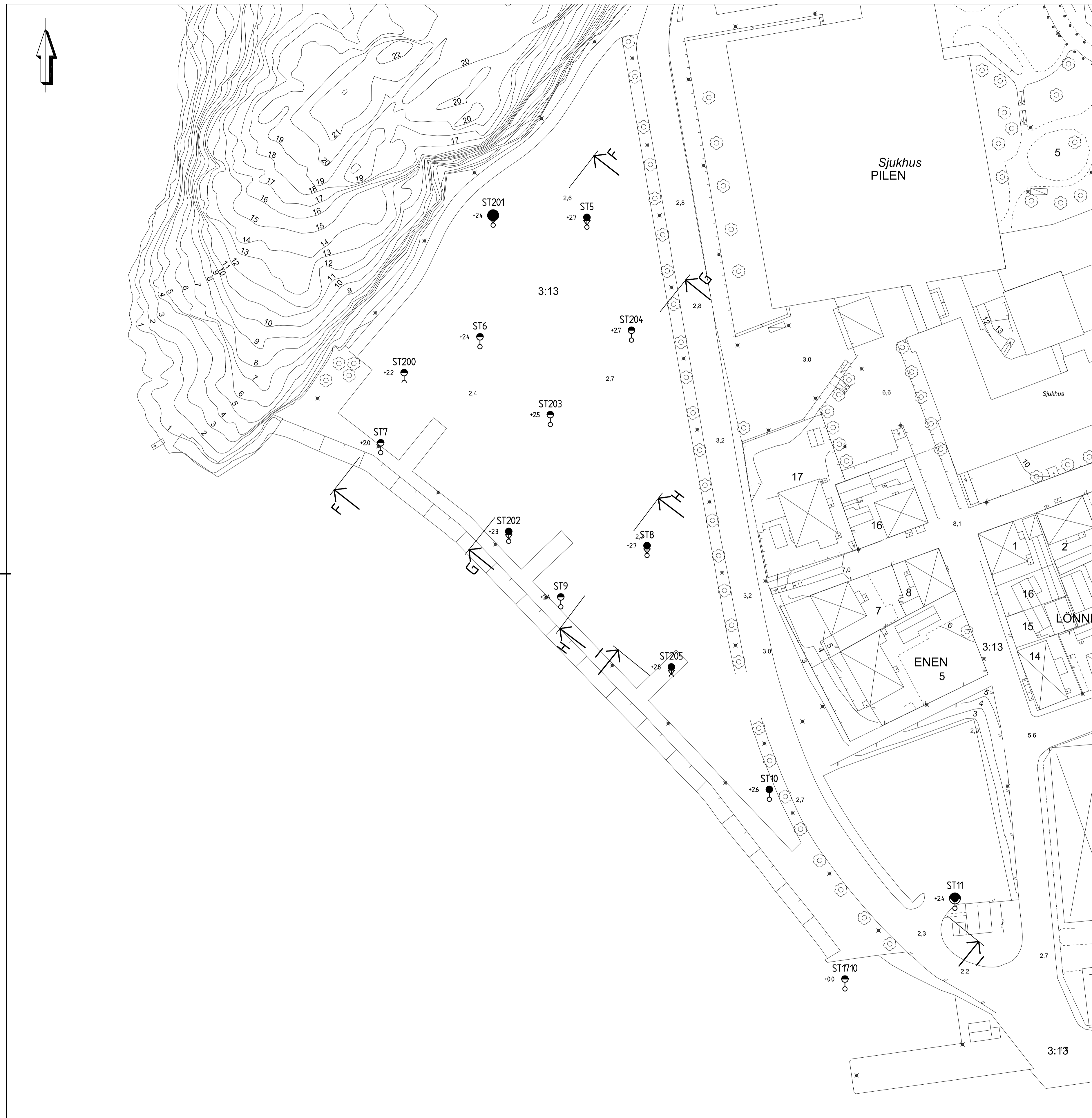
PLAN 1500 (A1)
